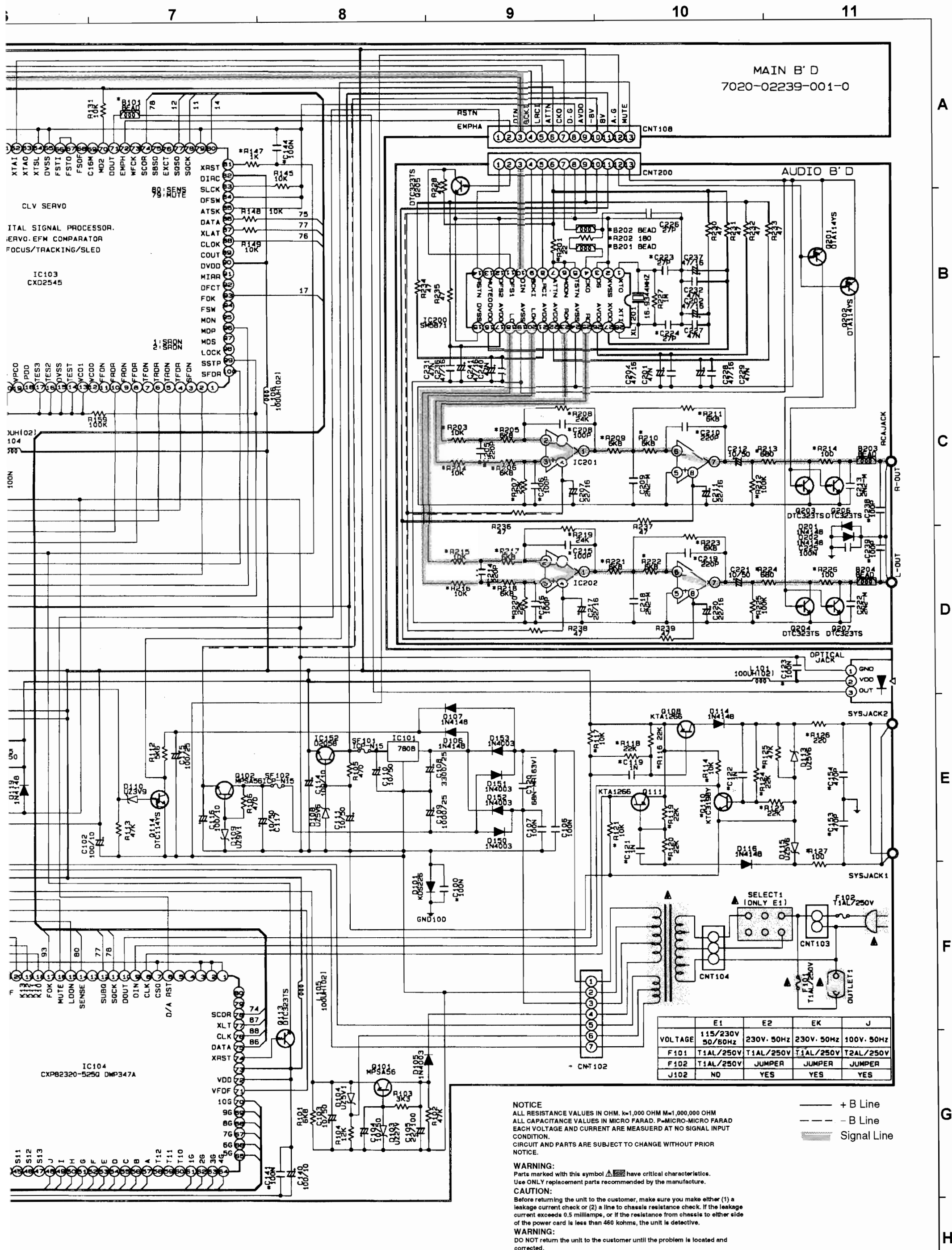
SCHEMATIC DIAGRAM MAIN P.W.B. UNIT
