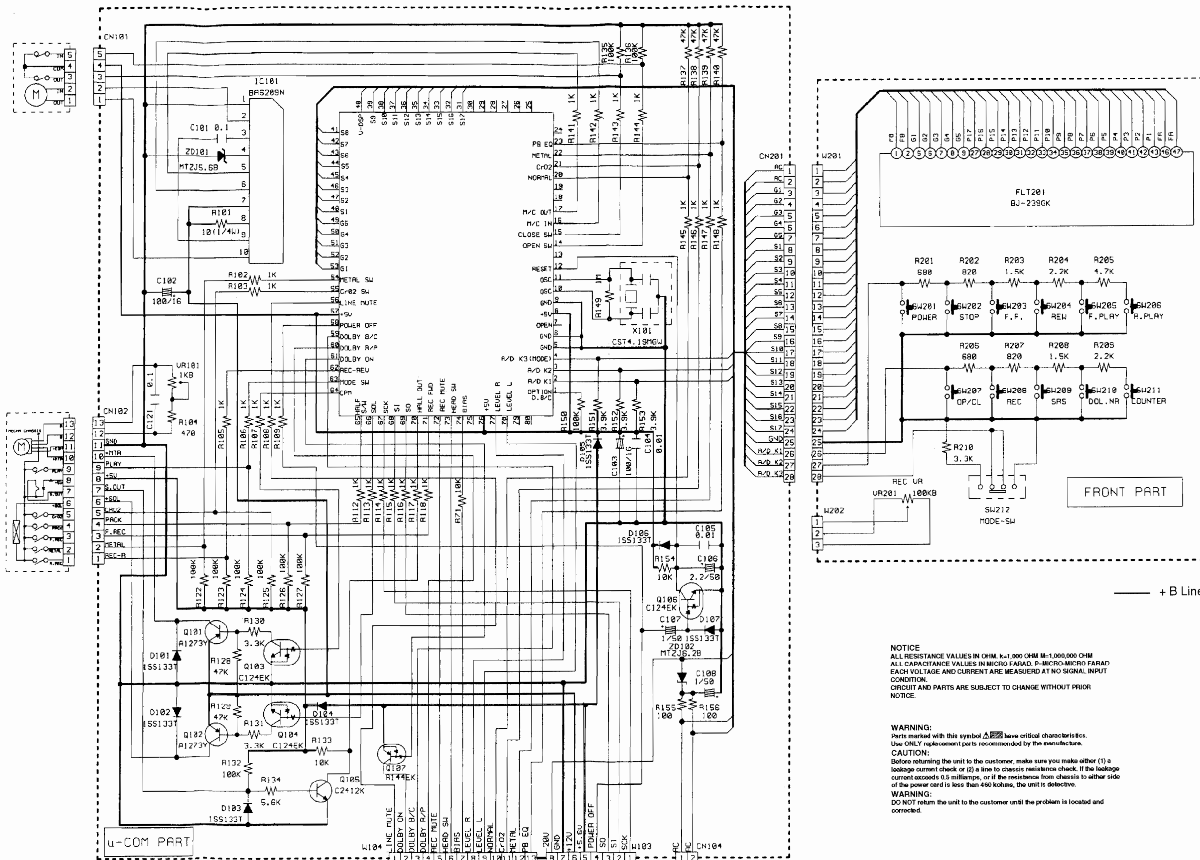
SCHEMATIC DIAGRAMS (2/2) FRONT / MICOM UNIT
